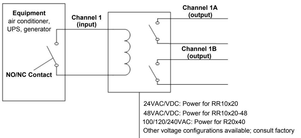
Schematic illustrating the use and placement of the Relay Replicator
