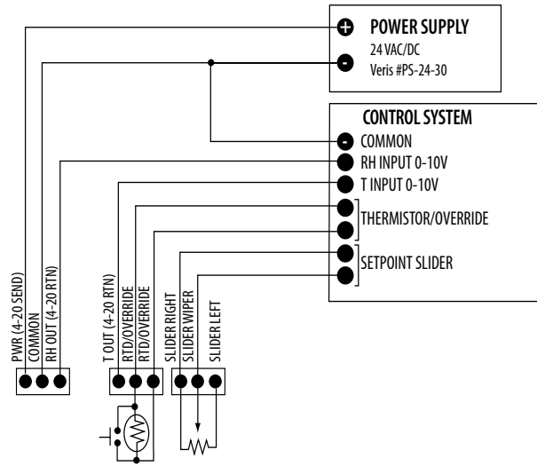
Voltage Output (3-Wire, 0-10V)
